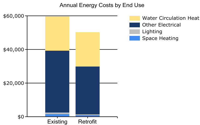
Figure 8: Annual energy costs by end use.
