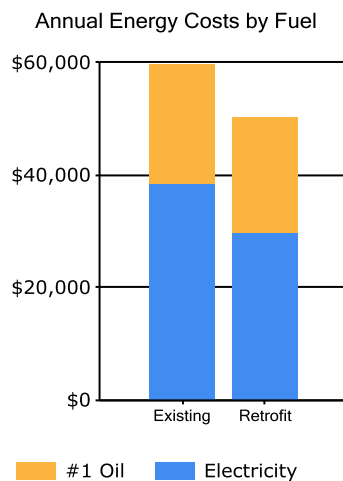
Figure 9: Annual energy costs by fuel type.
