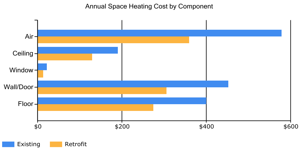
Figure 10: Annual space heating costs by component.
