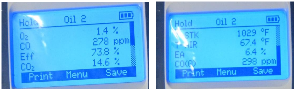
Figure 5: Boiler 1 combustion test results.
