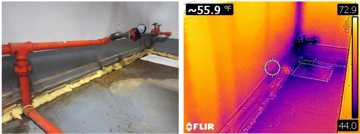
Figure 3: Evidence of differential movement between the floor and wall, thermal image.
