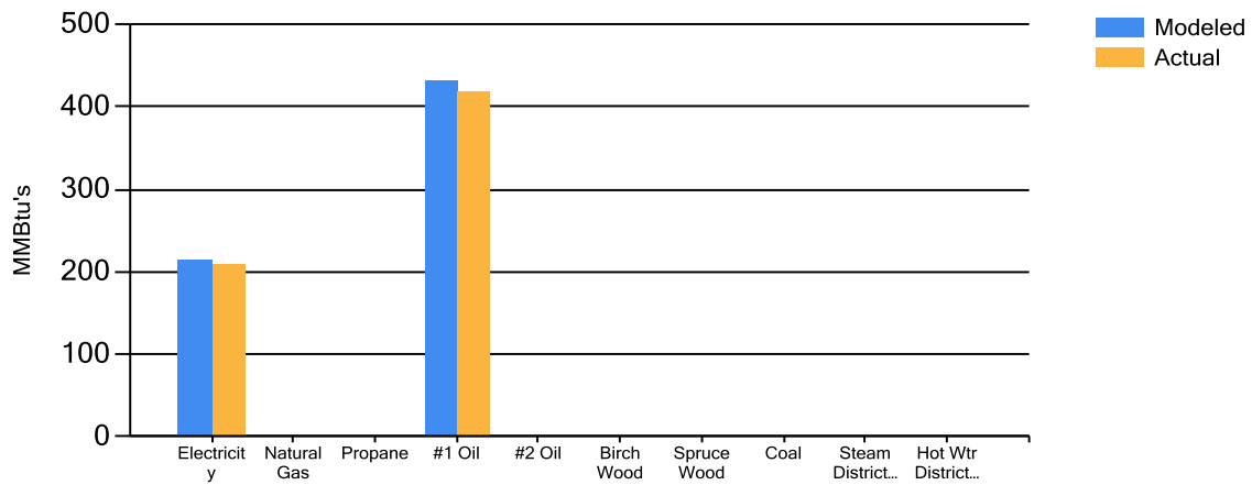
Electricity Use
