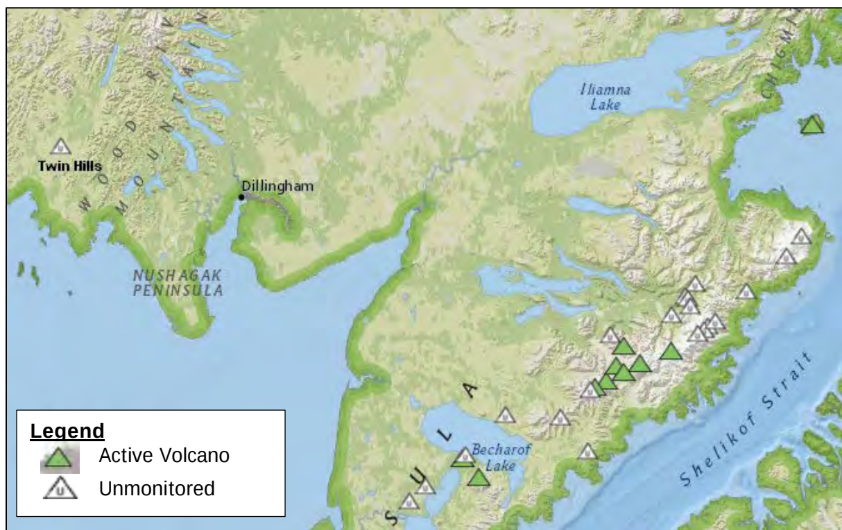
Exhibit 5-7: Volcanos Near Twin Hills
