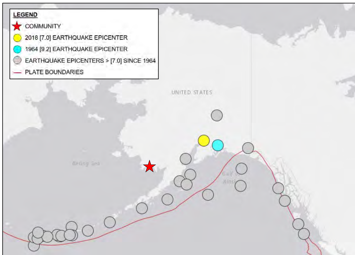
Exhibit 5-2: Major Earthquakes in Alaska
