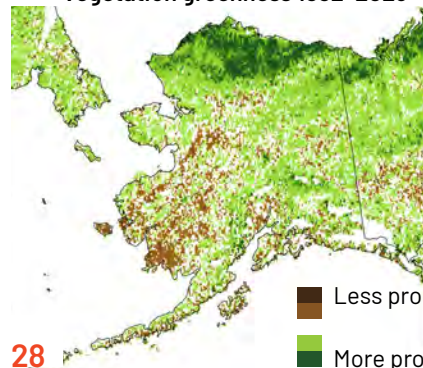
Vegetation greenness 1982–2023
