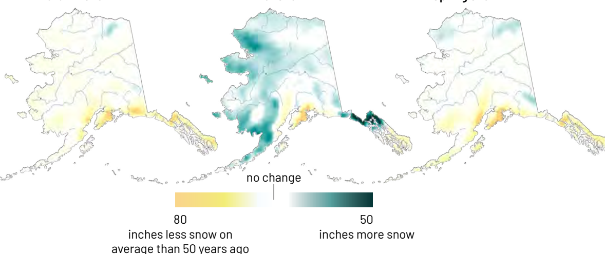
Autumn snow
