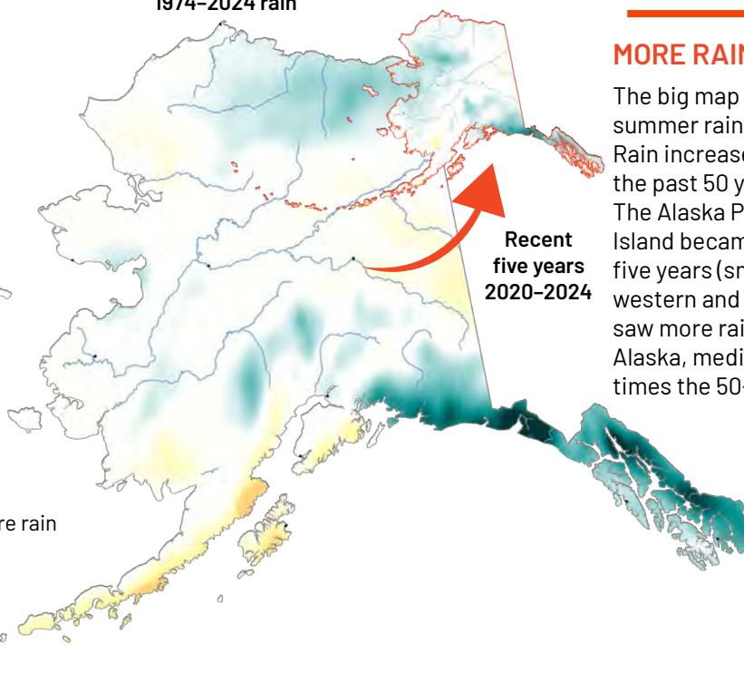
1974–2024 rain
