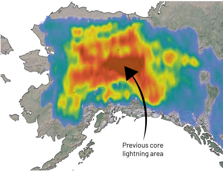
2004–2013 lightning
